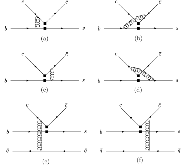
Fig. 1 Feynman diagrams for vertex and spectator corrections to B \rightarrow \chi_{c0}K .
